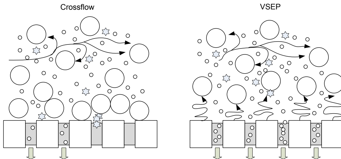
40 Fig. 1. The difference in colloid aggregation in cross flow filtration and VSEP (Image 41 adapted from Johnson) [3] 42
