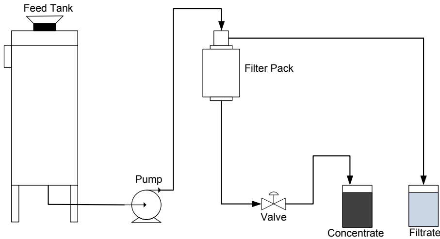
Fig. 2. The basic VSEP system setup (Imaged adapted from Culkin) [8]
