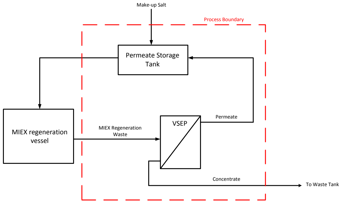
Fig. 3. A process flow diagram showing the system boundary of the installed VSEP established to conduct the economic analysis
