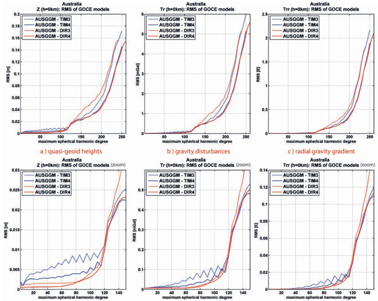
Fig. 4 RMS values computed from the differences of selected GOCE GGFMs and the newly retrieved AUS-GGM in terms of (a) quasi-geoid heights \zeta in meters [left], (b) gravity disturbances T_r in mGal [middle] and (c) radial gravity gradients T_{rr} [right] on the ellipsoid ( h = 0 ); the bottom row plots zoom into the respective upper plot in the degree range 0 to 150
