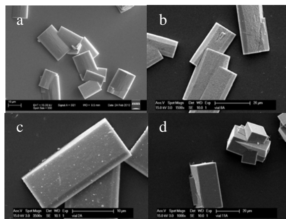
75 Fig. 2 SEM images of barium sulfate formed in the presence of (a) 0 mM tetrazole (b) 3.42 mM phtetH . (c) 2.45 mM mbtetH . (d) 2.47 mM phtet 2 H 2 .
