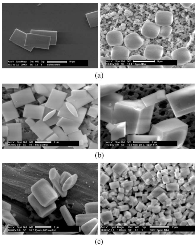
Fig. 5 Effect of temperature on morphology of barite particles formed (control and with 0.078 mM NTA). (a) 25 °C; (b); 60 °C; (c) 80 °C (all scale bars 2 μm, except top pictures which are 10 and 5 μm, respectively).
