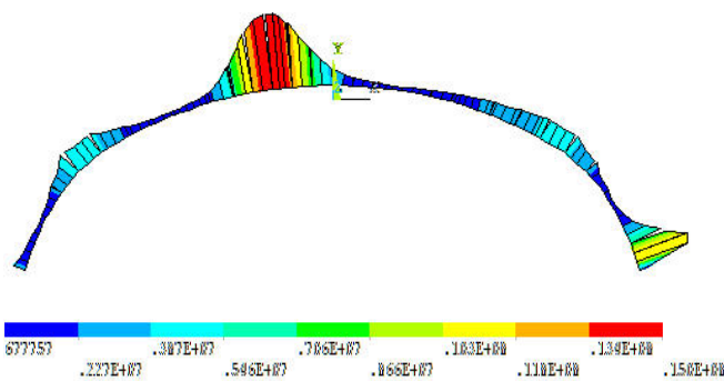
Fig. 4 – Strength demands on arch cross sections for a specific bogey location (N/m 2 )
