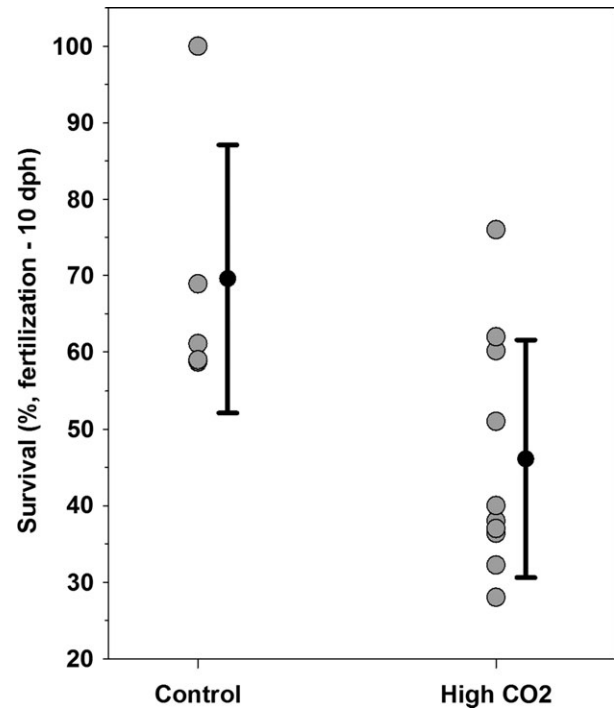
Figure 2 Menidia menidia . Survival from fertilization to 10 dph in offspring exposed to high (2300 \mu\text{atm} ) versus ambient (control: 460 \mu\text{atm} ) pCO_2 levels.
