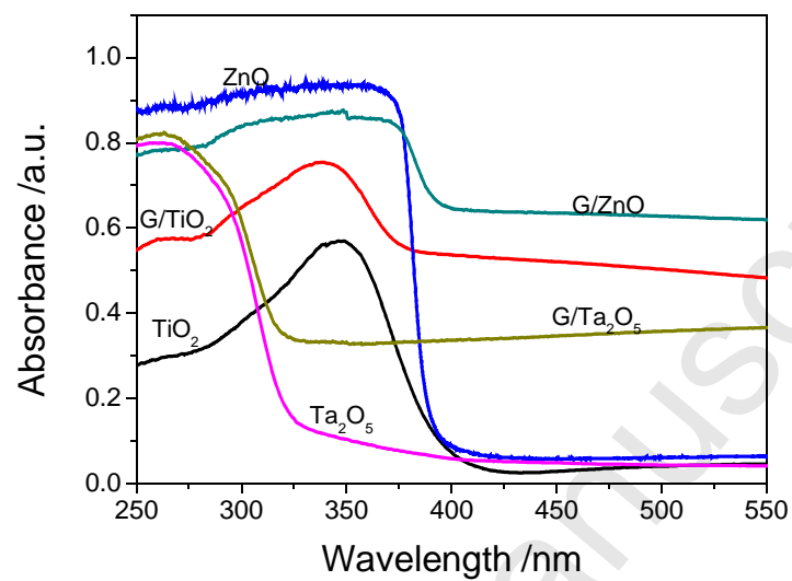
Fig. 5 UV-vis DRS of photocatalyst and their composites
