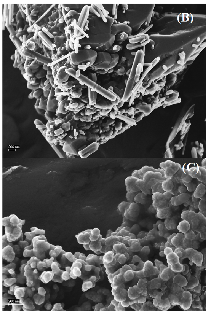
Fig. 2 SEM images of G/TiO 2 (A), G/ZnO (B), and G/Ta 2 O 5 (C).
