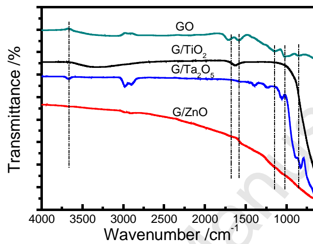
Fig. 4 FTIR spectra of GO and rGO/photocatalyst composites
