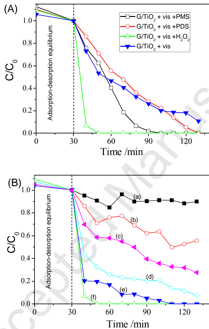
Fig. 7 Photochemical oxidation of methylene blue at various conditions. (A) Effect of oxidants, (B) Effect of amount of H 2 O 2 : (a) 0.338 mol/L H 2 O 2 only, (b) 0.338 mol/L H 2 O 2 and visible light, (c) G/TiO 2 and vis and 0.050 mol/L H 2 O 2 , (d) G/TiO 2 and vis and 0.147 mol/L H 2 O 2 , (e) G/TiO 2 and vis and 0.250 mol/L H 2 O 2 , and (f) G/TiO 2 and vis and 0.338 mol/L H 2 O 2 .
