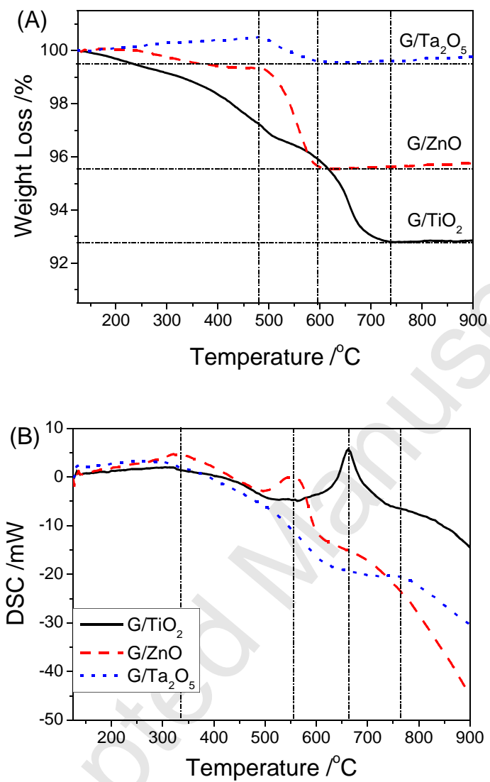
Fig. 3 TG/DSC diagram of the three composites of G/TiO 2 , G/ZnO and G/Ta 2 O 5
