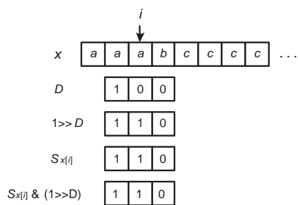
Figure 15. ShiftAnd-Matching Continues
