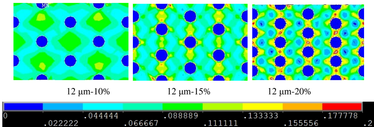
Fig. 15 von Mises total strains in composite with 12 \mu m diameter circular particles
