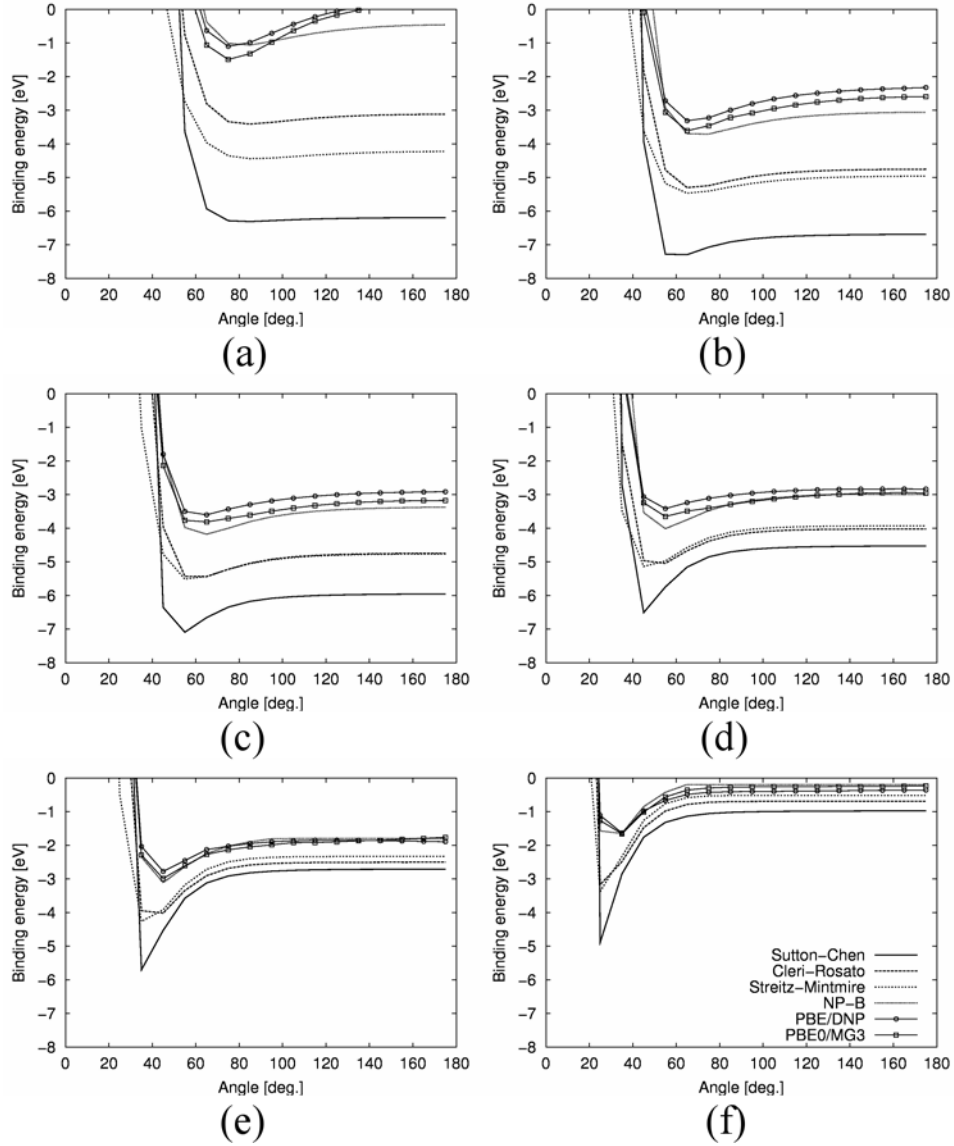
Figure 3: Binding energy of \text{Al}_3 as a function of angle at different r_1, r_2 separations: (a) r_1, r_2=2 \text{ \AA} , (b) r_1, r_2=2.3 \text{ \AA} , (c) r_1, r_2=2.506 \text{ \AA} , (d) r_1, r_2=2.863 \text{ \AA} , (e) r_1, r_2=3.5 \text{ \AA} , and (f) r_1, r_2=5 \text{ \AA} .
