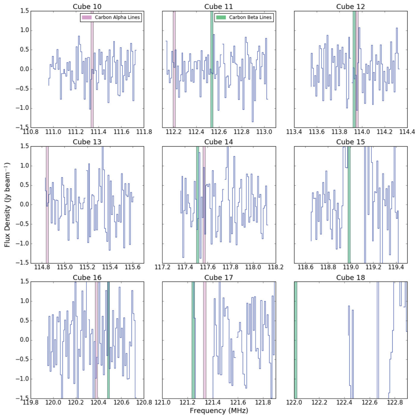
Figure A6. MWA spectra for a data cube used within this survey at the position of G194.67 –23.76. The alpha recombination rest frequency positions are marked in plum and the beta rest frequency positions are marked in green. Flagged channels are blanked out in the spectra.
