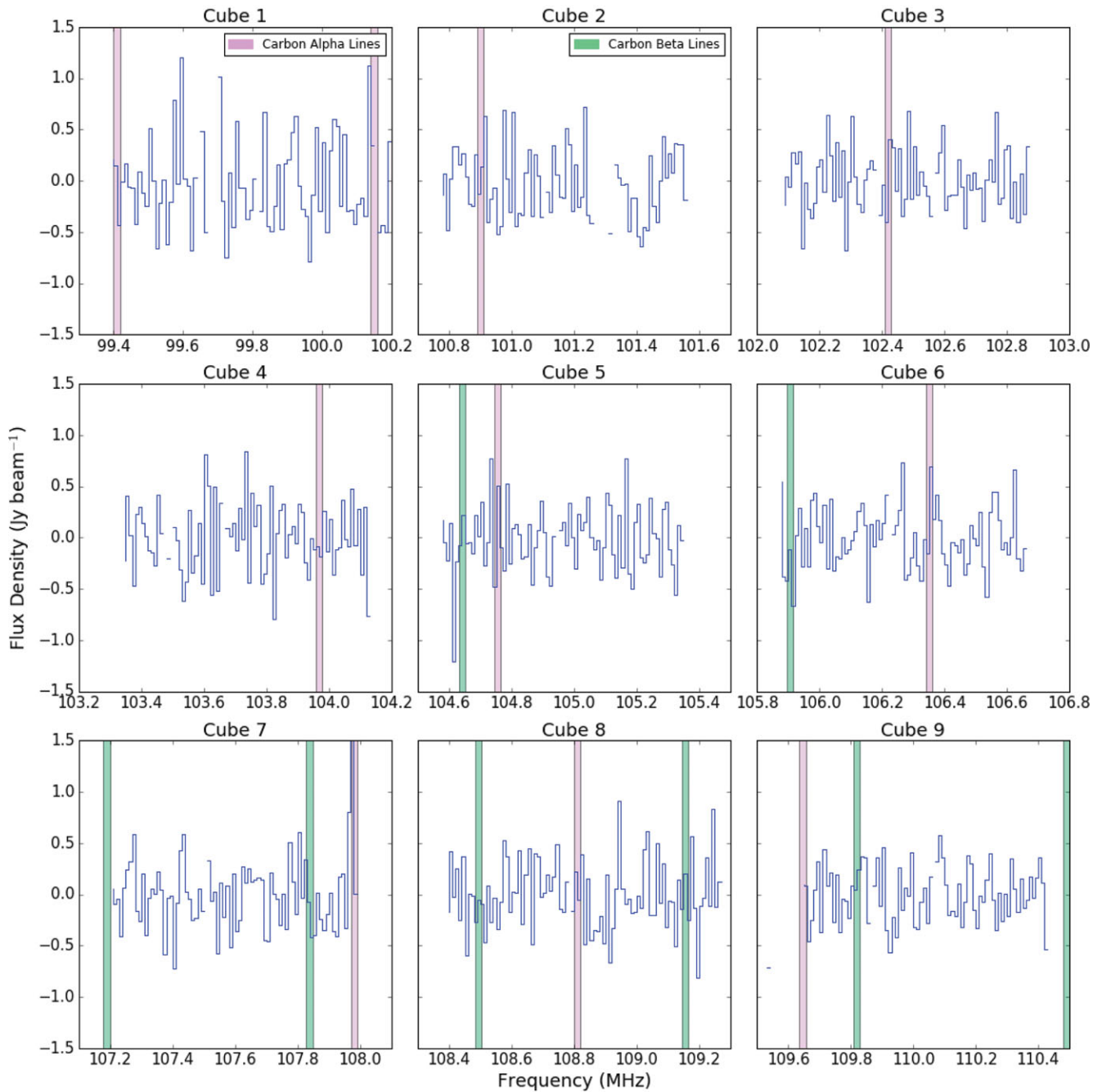
Figure A3. MWA spectra for a data cube used within this survey at the position of G194.67 –23.76. The alpha recombination rest frequencies are marked in pink and the beta rest frequency positions are marked in green. Flagged channels are blanked out in the spectra.
