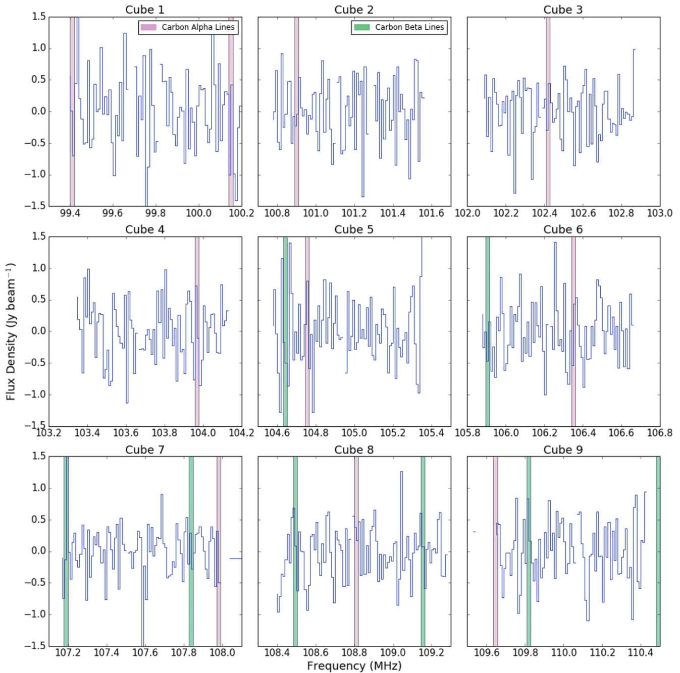
Figure A5. MWA spectra for a data cube used within this survey at the position of G194.67 –23.76. The alpha recombination rest frequencies are marked in pink and the beta rest frequency positions are marked in green. Flagged channels are blanked out in the spectra.
