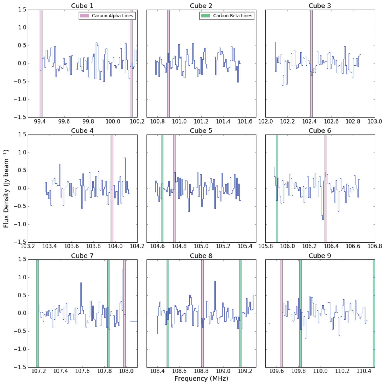
Figure A1. MWA spectra for a data cube used within this survey at the position of G212.67 –25.56. The alpha recombination rest frequency are marked in plum and the beta rest frequency positions are marked in green. Flagged channels are blanked out in the spectra.
