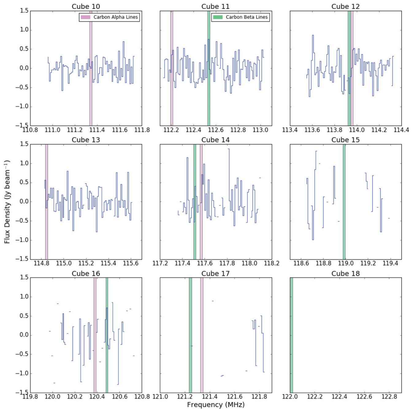
Figure A4. MWA spectra for a data cube used within this survey at the position of G210.67 – 10.75. The alpha recombination rest frequency positions are marked in plum and the beta rest frequency positions are marked in green. Flagged channels are blanked out in the spectra.
