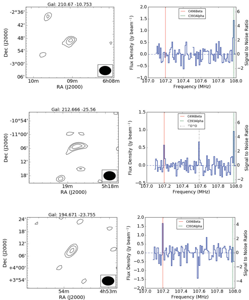
Figure 2. A tentative detection of the C393 \alpha (107.98 MHz) and C496 \beta (107.19 MHz) at the Galactic coordinates listed on the top of each plot. The contours plot on the left represent the 3, 4, 5, and 6 \sigma levels of the associated detection. The spectrum on the right is representative of the spectrum of the coarse channel band in which the tentative detection was made with the flagged channels blanked. The spectra at G212.67 –25.56 also shows a possible detection of C496 \beta at 107.18 MHz and molecular oxygen ( ^{17}\text{O}^{18}\text{O} ) at 107.60 MHz.
