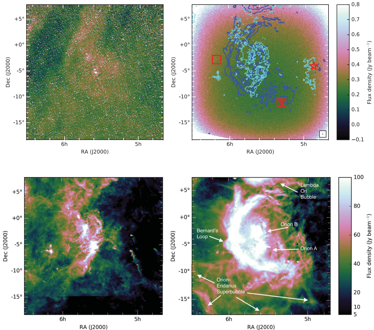
Figure 1. The upper left image is a continuum image of the Orion survey region across the 30.72 MHz of bandwidth with a central frequency of 114.6 MHz showing the full region blindly searched for molecular signatures and recombination lines. The upper right-hand image is an RMS map showing the sensitivity of the MWA in a typical coarse channel data cube. The C393 \alpha and C496 \beta transitions are represented by squares and stars, respectively. The contours in cyan trace the image in the bottom left, which shows dust emission at 100 \mu\text{m} surveyed by Schlegel et al. (1998). The blue contours and the image in the bottom right are the optical H \alpha emission from the Southern H-Alpha Sky Survey Atlas (SHASSA) (Finkbeiner 2003). We note that there is an image artefact in the 100 \mu\text{m} survey data on the bottom, created by combining the data from different fields.
