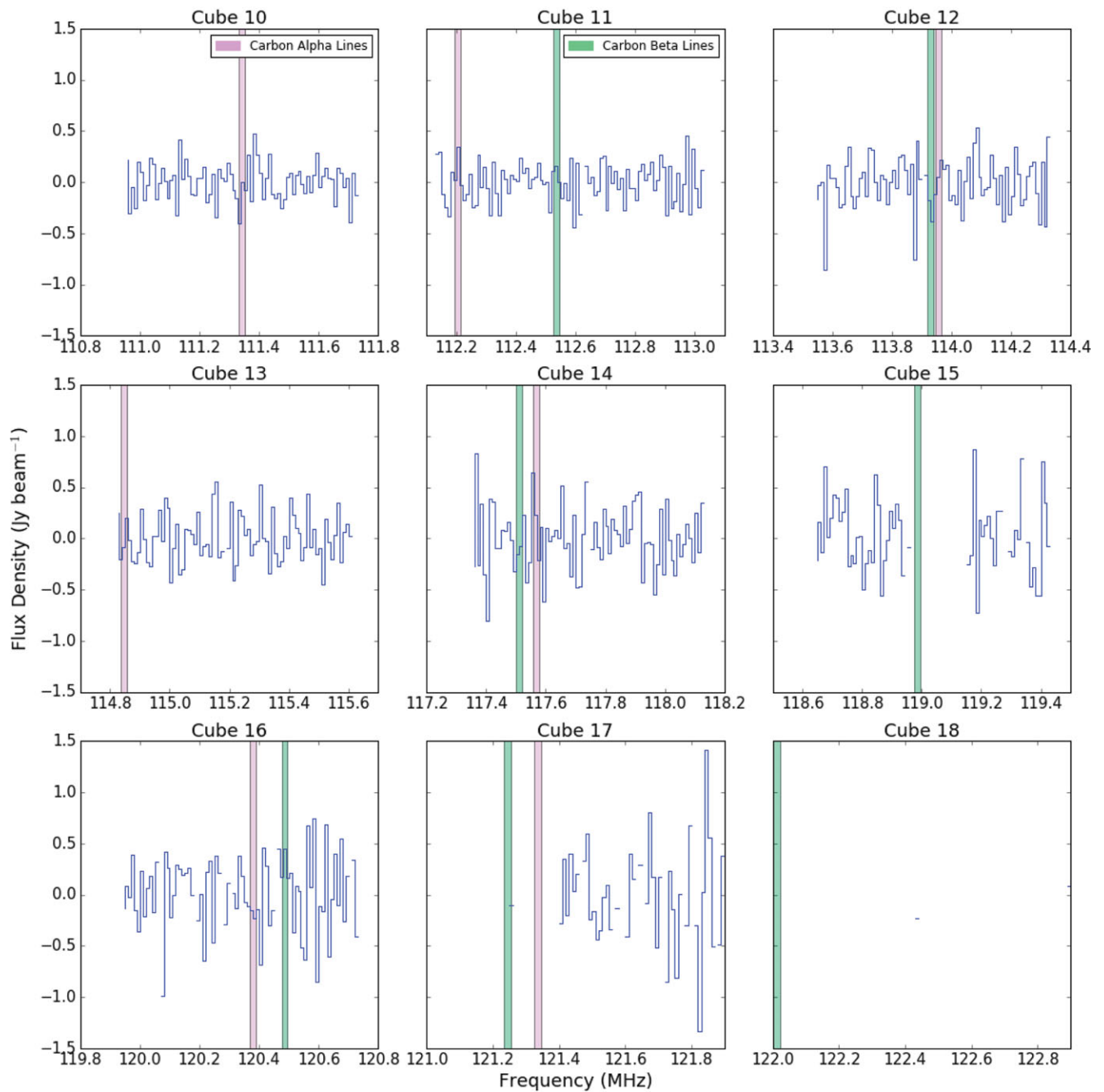
Figure A2. MWA spectra for a data cube used within this survey at the position of G212.67 –25.56. The alpha recombination rest frequency positions are marked in plum and the beta rest frequency positions are marked in green. Flagged channels are blanked out in the spectra.
