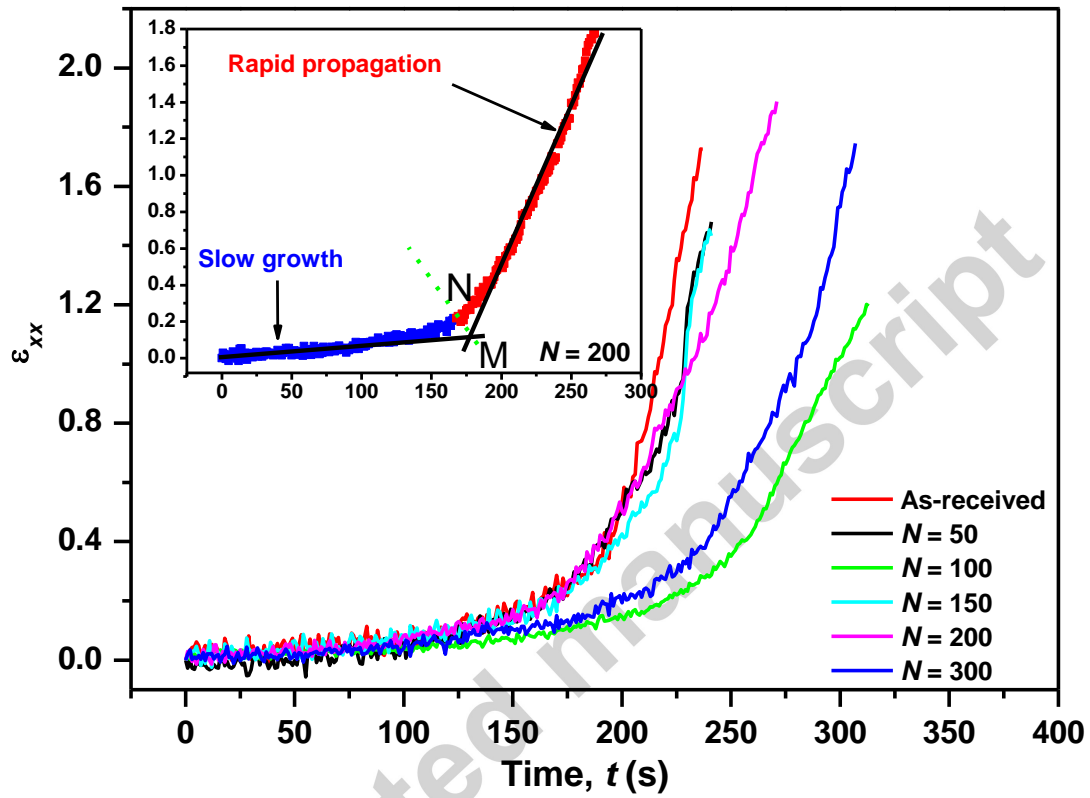
Fig. 4 The relationship of \epsilon_{xx} by DIC in the monitored region versus loading time during bending tests.
