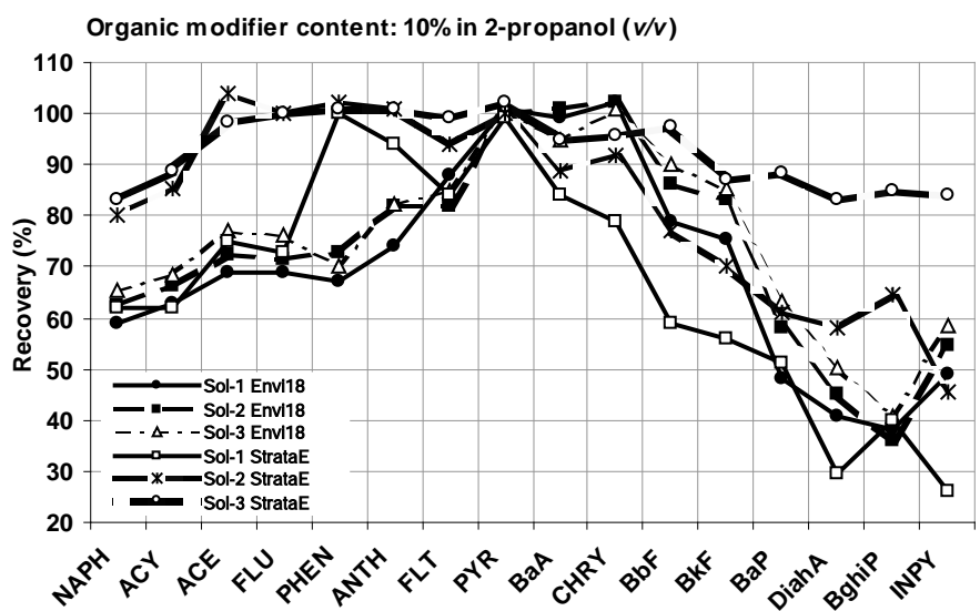
1 FIGURE 7. Percentage recoveries (n=3) achieved using 10% of 2-propanol in spiked 2 Milli-Q water samples (1000 mL, 100 ng/L spiking level except for NAPH and ACY: 3 1000 ng/L) and by varying the best stationary phases (StrataE and Envi-18) and the 4 eluting mixtures (Sol-1, Sol-2 and Sol-3).
