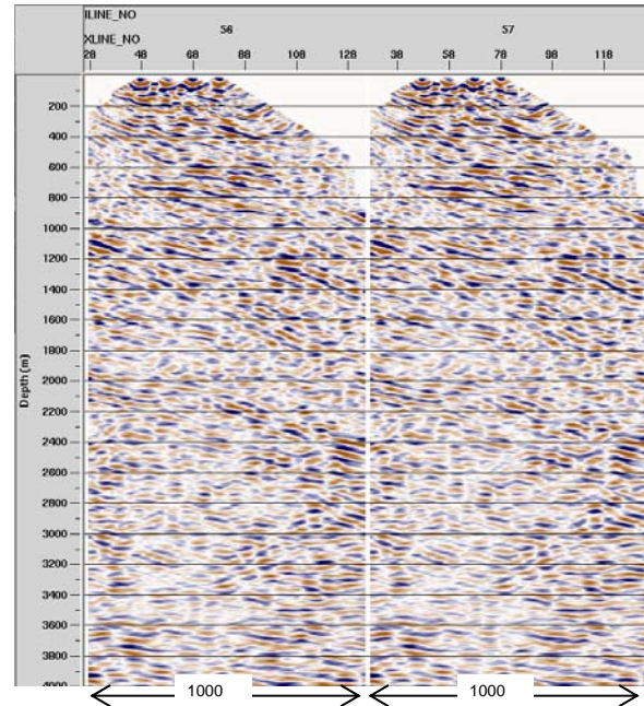
Figure 4. Pilot 3D study: inline stacks 56 and 57 converted to depth. Strong reflections at around 600 m depth correspond to the expected Nickel deposits at this site.
