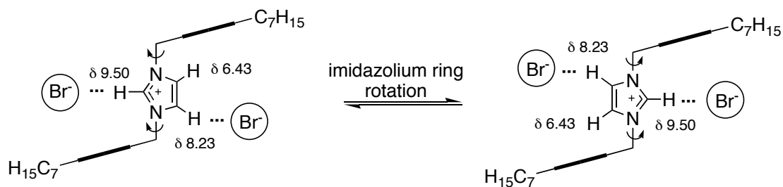
Figure 7. The predominant conformers in CD 2 Cl 2 solution of 8.2Br and the imidazolium ring rotation process that converts the two conformers.
