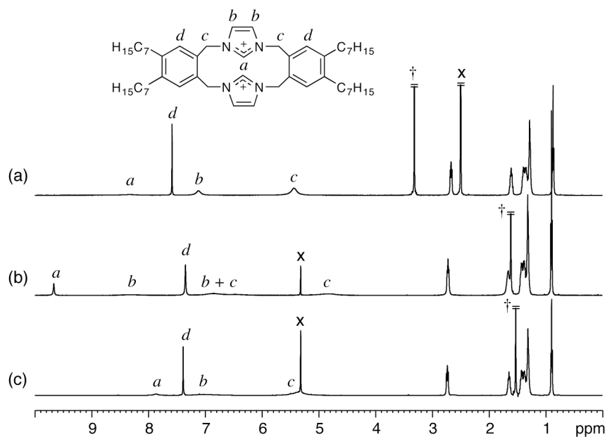
Figure 2. ^1\text{H} NMR spectra (500.1 MHz) of (a) 8.2Br in \text{DMSO-}d_6 , (b) 8.2Br in \text{CD}_2\text{Cl}_2 , and (c) 8.2PF 6 in \text{CD}_2\text{Cl}_2 , all recorded at 25 °C. Key: x = residual solvent signals, † = \text{H}_2\text{O} .
