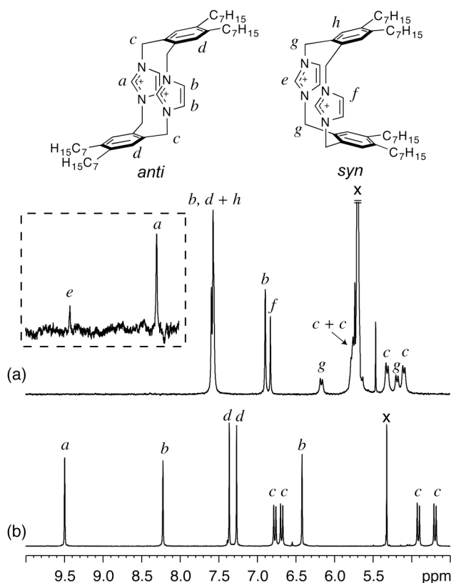
Figure 3. Downfield region of the ^1\text{H} NMR spectra (500.1 MHz) of 8.2Br (a) in \text{CD}_3\text{OD} at -70\text{ }^\circ\text{C} and (b) in \text{CD}_2\text{Cl}_2 at -40\text{ }^\circ\text{C} . The region shown in the dashed box is of a spectrum of 8.2Br in \text{CH}_3\text{OH} at -70\text{ }^\circ\text{C} indicating signals for the H2 protons. Key: x = residual solvent signals.
