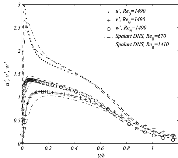
Fig. 5 Time and spanwise-averaged data for Re_\theta = 1490 : a) mean velocity profile and b) velocity fluctuation profile.
