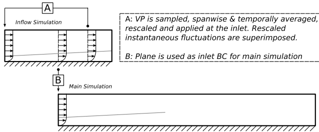
Fig. 1 Recycling inflow generation method.
