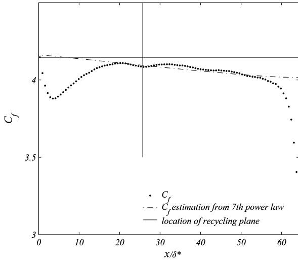
Fig. 4 Time and spanwise-averaged C_f(\times 10^3) in a streamwise direction, with inlet mirroring.
