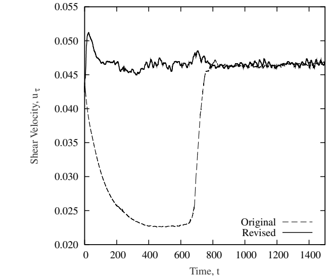
Fig. 6 Development of u_\tau over time at the inlet; original vs revised initial conditions.
