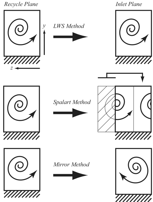
Fig. 3 Methods for disrupting error accumulation.
