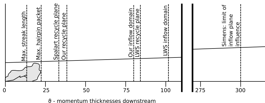
Fig. 2 Illustration of various LWS-based inflow simulation configurations, compared with the lengths of instantaneous boundary-layer structures. This illustration is intended to highlight relative scales.
