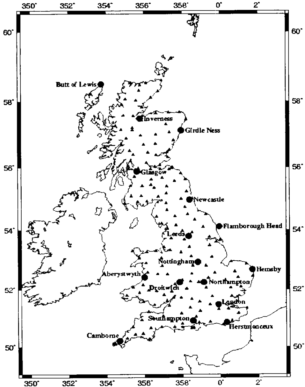
Fig. 1. The active stations (denoted by circles) and the FBM stations (denoted by triangles) distributed across the British mainland
