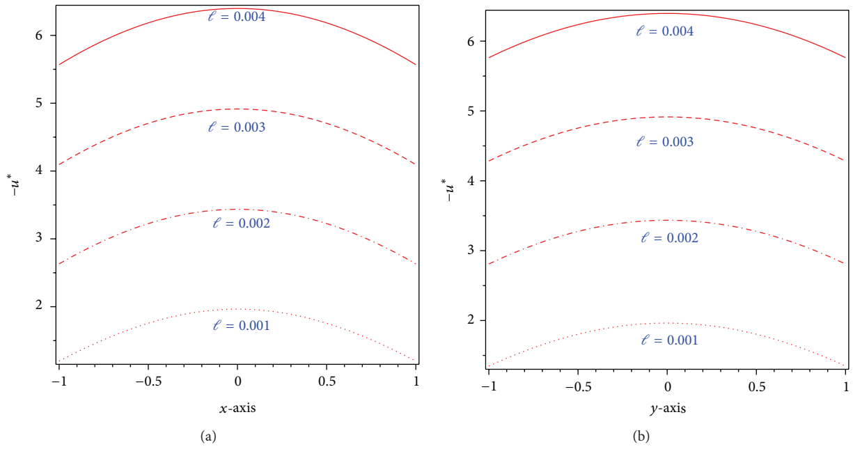
FIGURE 4: 2D velocity profile along the x-axis and y-axis on the cross-section of the channel with the area of 1.0 \times 10^{-6} \text{ m}^2 and ratio \epsilon of 3/4 for constant pressure gradient under different slip lengths \ell values.
