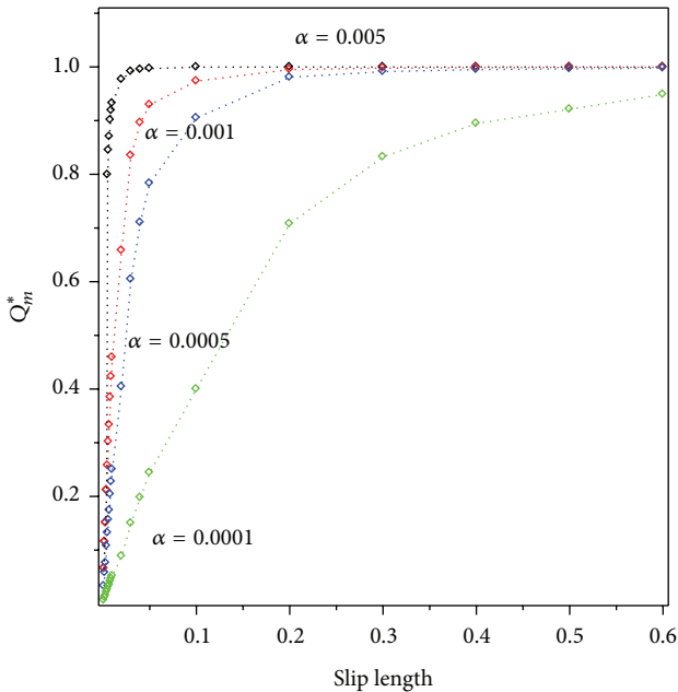
FIGURE 9: Influence of slip length on the amplitude of the flow rate Q_m^* on the cross-section of the channel with the area of 1.0 \times 10^{-6} \text{ m}^2 and ratio b/a of 1 under different frequencies \omega = \alpha/\rho a^2 with different \alpha .
