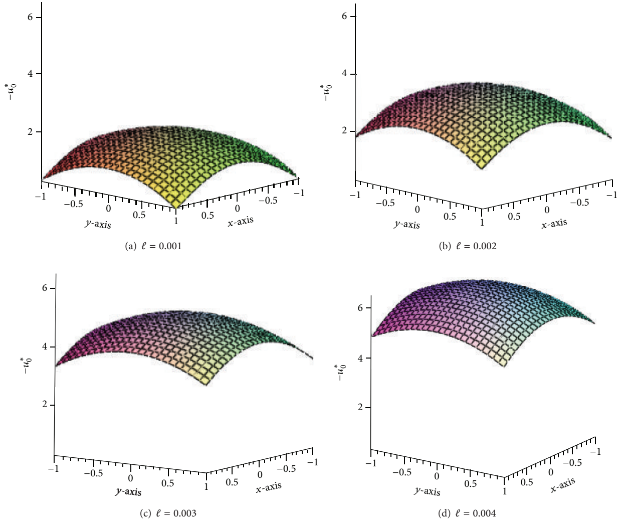
FIGURE 3: Axial velocity profile on the cross-section of the channel with the area of 1.0 \times 10^{-6} \text{ m}^2 and ratio \varepsilon of 3/4 for constant pressure gradient under various values of slip lengths \ell : (a) \ell = 0.001 ; (b) \ell = 0.002 ; (c) \ell = 0.003 ; (d) \ell = 0.004 .
