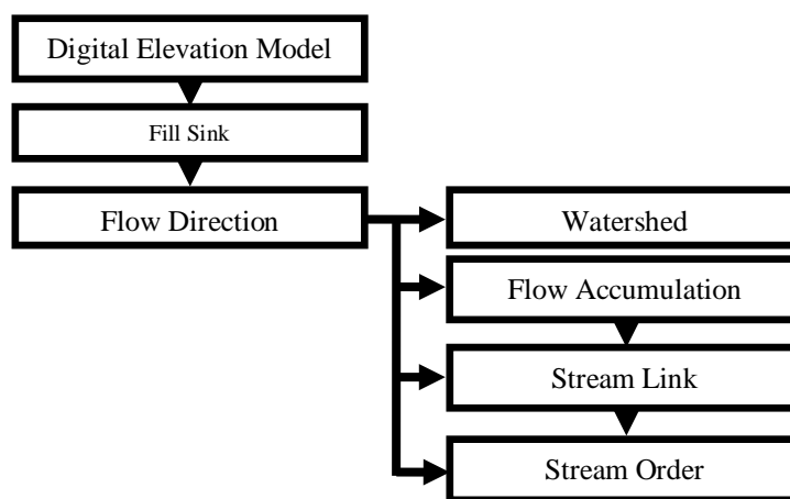
Figure 3. Watershed Modeling
