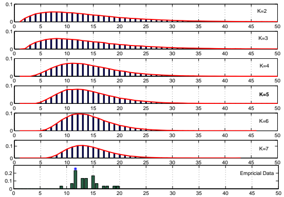
Fig. 11. (continue from Fig. 10) Learned Coxian with increasing number of phases from 2 to 7 for “at-sink” in activity (a.3).
