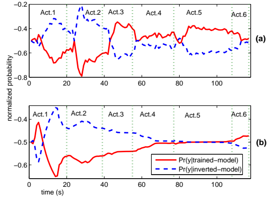
Fig. 16. Abnormality detection with: (a) the 5-phase CxSHSMM and its 2-phase \bar{D}_{p,i} counter model, and (b) the flat HSM and its “inverted” duration counter model.
