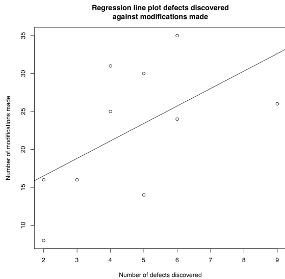
Figure 4. Scatterplot demonstrating the relationship between discovering defects and modification ability.
