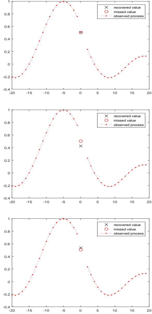
Figure 1: Example of a path x \in \ell_2^{BL, \Omega} with \Omega = 0.1\pi and the recovered values \hat{x}(0) calculated using 100 observations: (i) calculated by (6) for \Omega = 0.1\pi (top); (ii) calculated by (6) with \Omega = 0.05\pi (middle); (iii) calculated by (10) (bottom).
