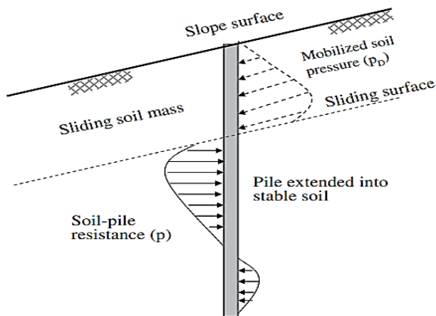
Figure 5: Driving force induced by displaced soil mass above the sliding surface (Ashour and Ardalán, 2012)
