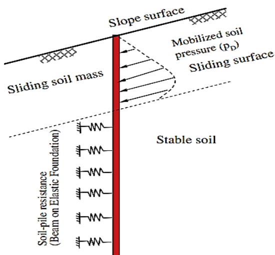
Figure 6: Proposed model for soil-pile analysis in pile stabilized slopes (Ashour and Ardalán, 2012)
