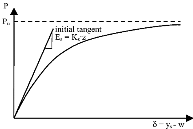
Figure 3: Hyperbolic P-δ curve (Jeong et al., 2003)
