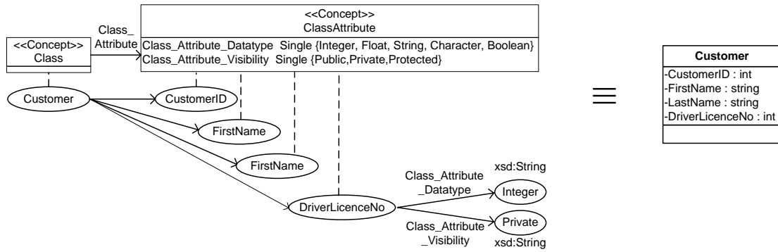
Figure 5 Transformation of UML class Customer and its attributes to class diagrams
