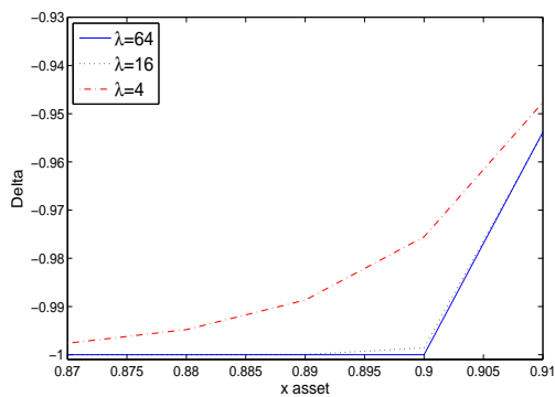
Figure 2: American put option Delta at t = 0 , computed by l_2 penalty method with three penalty parameter \lambda = 4, 16, 64 , data as in Table 1. Grid: 640 \times 640 , time steps = 200.
