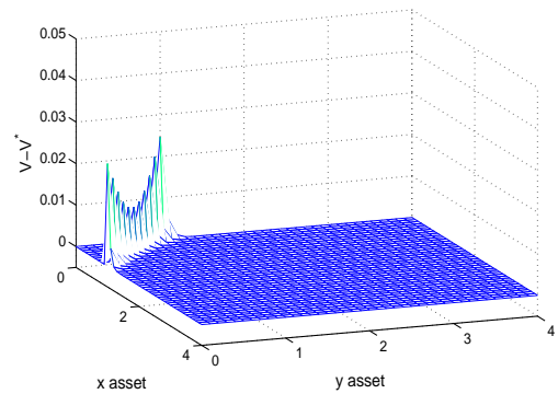
Figure 5: V - V^* computed at t = 0 by l_2 penalty method with \lambda = 32 . Grid: 640 \times 640 , time steps = 200.
