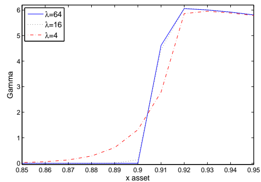
Figure 3: American put option Gamma at t = 0 , computed by l_2 penalty method with three penalty parameter \lambda = 4, 16, 64 , data as in Table 1. Grid: 640 \times 640 , time steps = 200.
