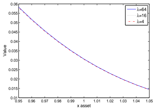
Figure 1: American put option value at t = 0 , computed by l_2 penalty method with three penalty parameter \lambda = 4, 16, 64 , data as in Table 1. Grid: 640 \times 640 , time steps = 200.
