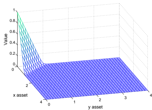
Figure 4: V computed at t = 0 by l_2 penalty method with \lambda = 32 . Grid: 640 \times 640 , time steps = 200.
