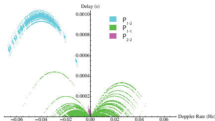
Figure 2. A schematic of the secondary spectrum of PSR 0834+06 found by Brisken et al. (2010). The green points represent interference between speckles on the primary scattering disk, cyan represents interference between speckle pairs on the primary disk with those on the secondary scattering disk, and the purple points represent interference between adjacent speckles on the secondary scattering disk.
