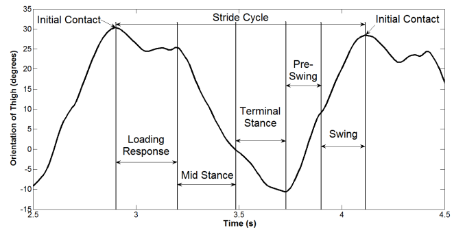
Figure 5. Gait Phases Identified Based on Thigh Angle
