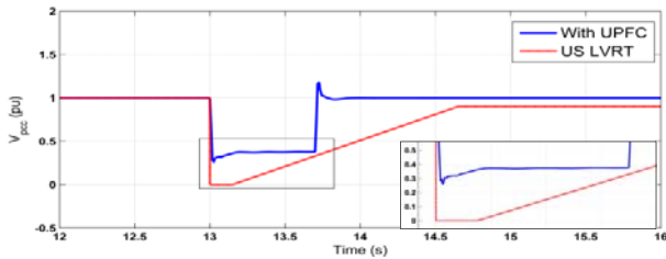
Fig. 13. DFIG compliance with US LVRT with UPFC
