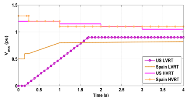
Fig. 1. FRT grid codes of Spain and US
