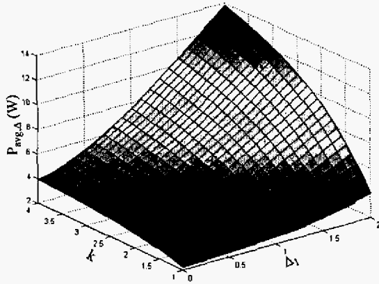
Fig. 5. Surface P_{avg,\Delta}
