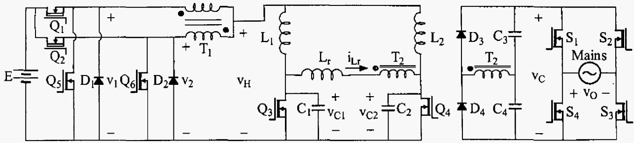
Fig. 2. The ZVS two-inductor boost converter with an unfold
