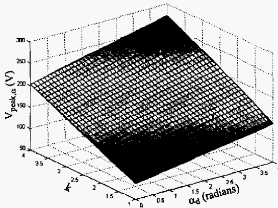
Fig. 7. Surface V_{peak,\alpha}
