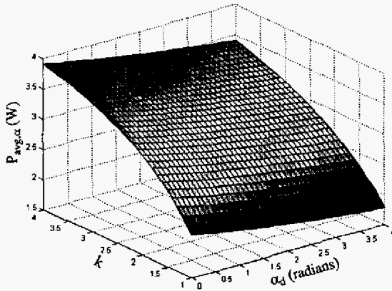
Fig. 6. Surface P_{avg,\alpha}
