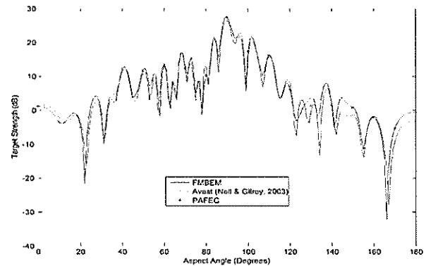
Figure 6. Monostatic target strength as a function of angle for the BeTSSi submarine at a frequency of 200Hz.
