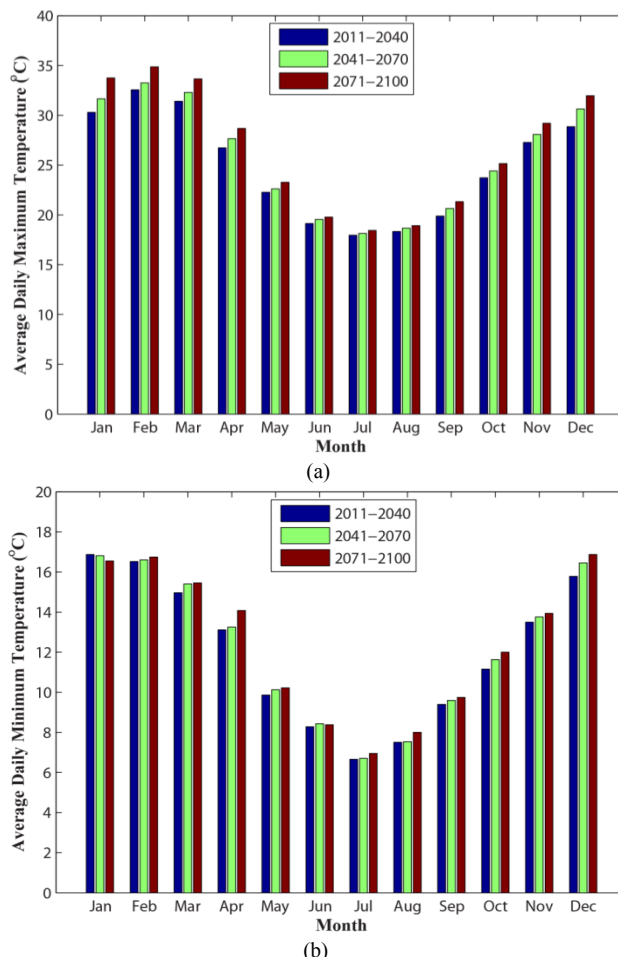
Fig. 10. Prediction of future daily average maximum and minimum pavement temperature.
