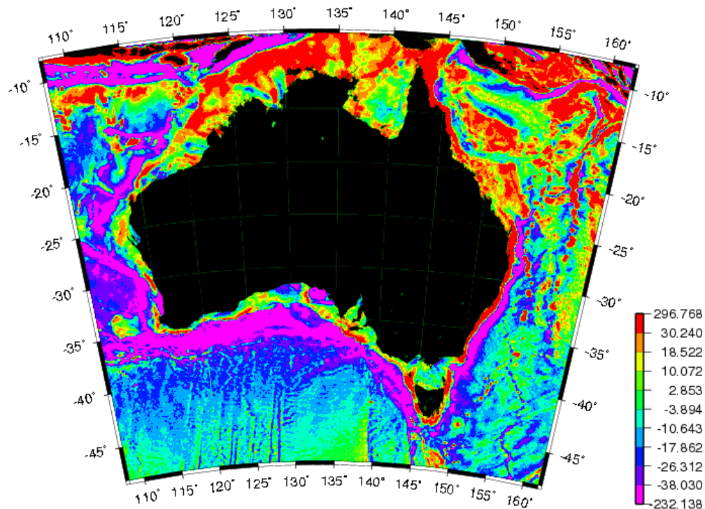
Figure 4. Marine gravity anomalies around Australia derived from multi-mission satellite radar altimetry (units in mGal; Lambert conformal conical projection)
