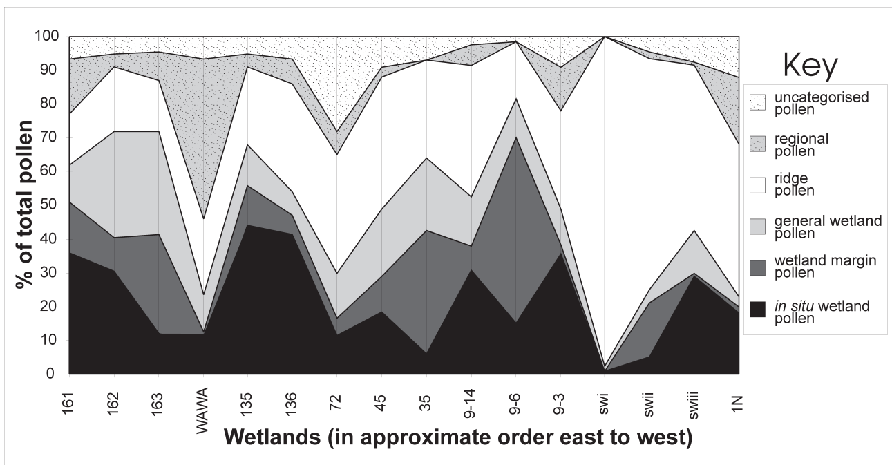
Figure 3. Composition of surface pollen for all sites.
