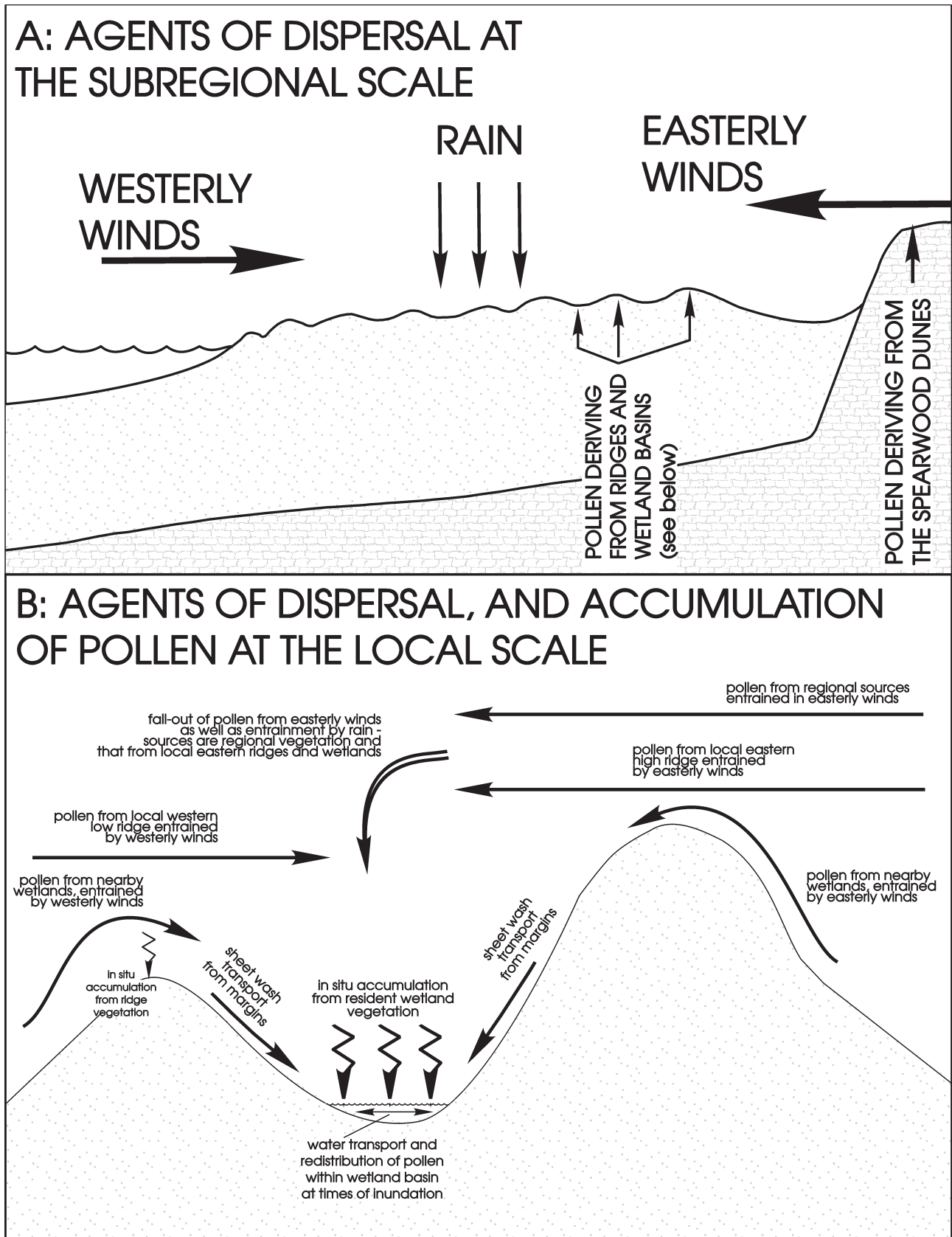
Figure 2. Potential patterns of dispersal and accumulation of pollen into wetland basins with in situ , local, and regional sources.
