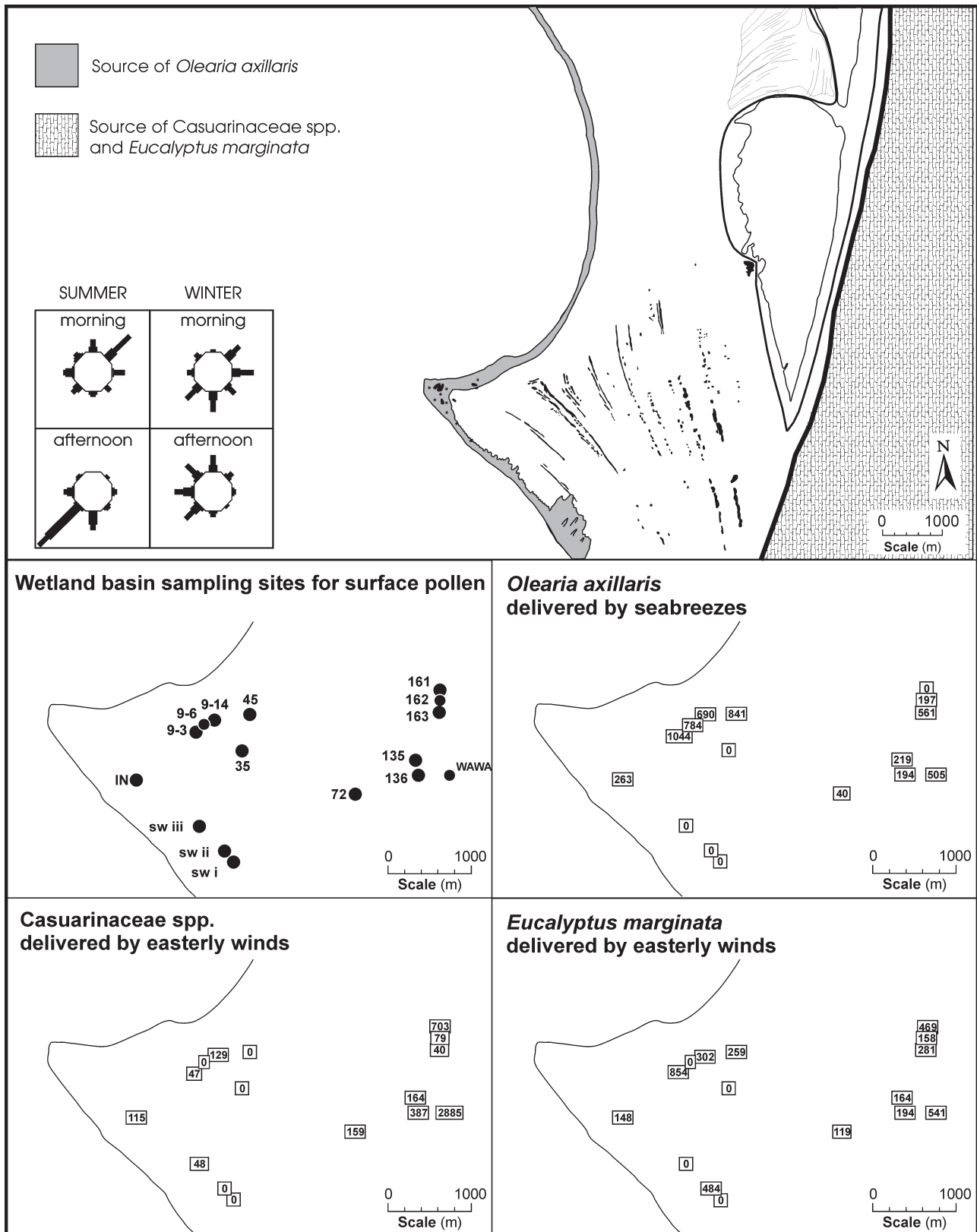
Figure 6. Sources of the three types of upland pollen ( viz. , O. axillaris , E. marginata , and Casuarinaceae spp, with source being coastal, and inland regional, respectively), summary of wind delivery systems shown as wind roses for summer and winter, and abundance of these pollen in the surface sediments of the wetlands (boxed numbers refer to number of pollen within a standard volume; see text). The regional sources for E. marginata include that shown in the Figure (the Spearwood Dunes), as well as sources further east, such as the Bassendean Dunes and the Darling Plateau.
