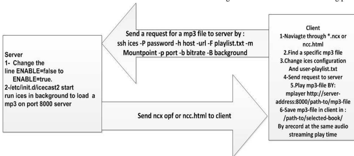
Fig. 2. DAISY streaming procedure
