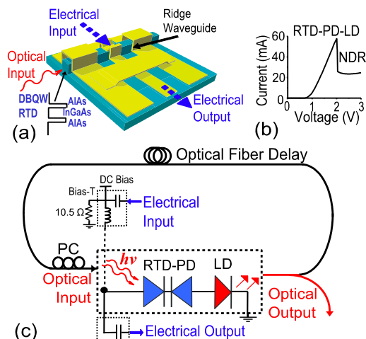
Fig. 6. (a) Shows the chip layout of the waveguide RTD photodiode (RTD-PD) (b) shows the current-voltage characteristic of the RTD-PD and laser diode combination (RTD-PD-LD), (c) shows the layout of the RTD-OEO and schematics of the electrical and optical output.
