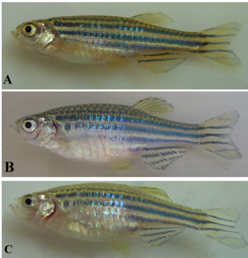
Figure 1. An illustration of a male zebrafish (A) and female zebrafish (B, C).
