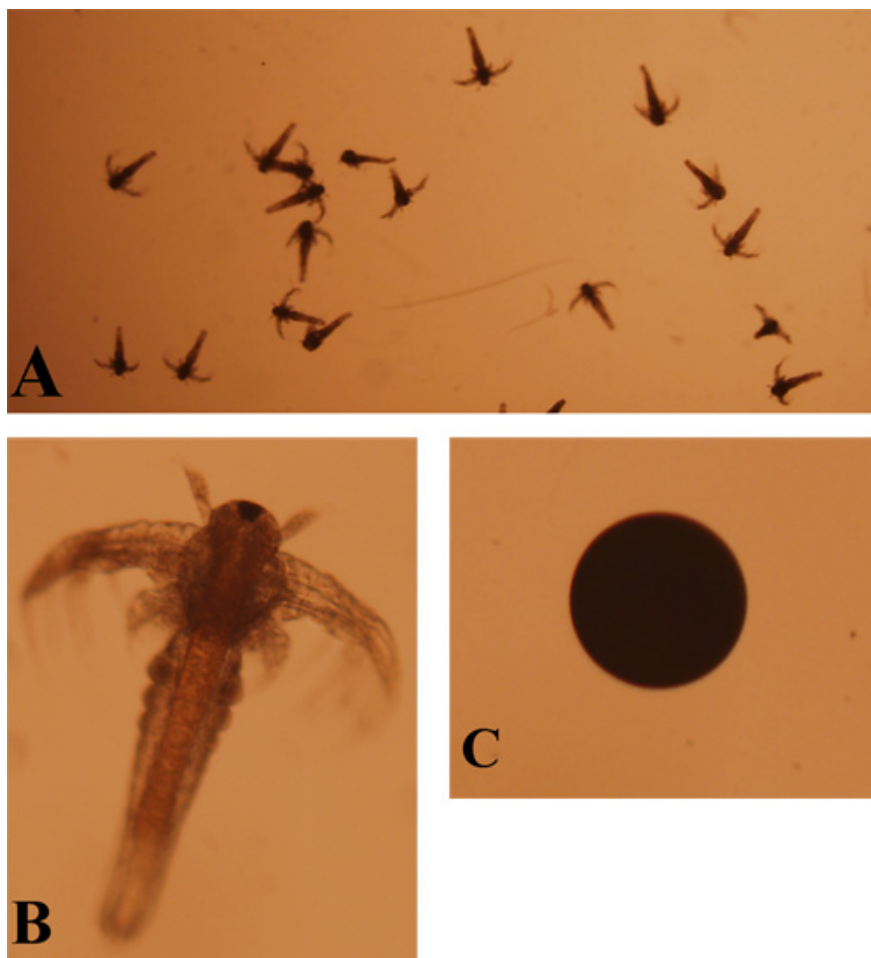
Figure 2. A microscopic view of brine shrimps at 12X (A), a single brine shrimp at 90X (B), and an unfertilized brine shrimp egg at 90X (C).
