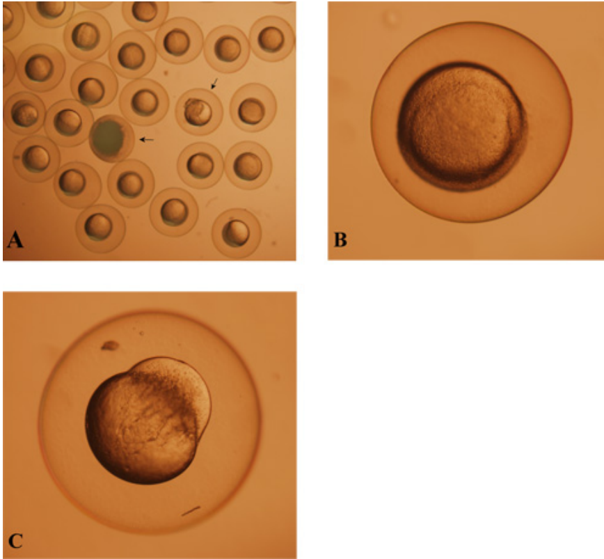
Figure 3. Microscopic view (16X) of fertilized and unfertilized eggs, where only two eggs are unfertilized, the unfertilized eggs are indicated with black arrows (A). Higher magnification view (90X) of a fertilized (B) and an unfertilized egg (C).
