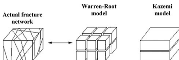
Fig. 1 Dual porosity–dual permeability system (Warren-Roort and Kazemi simplified models)
