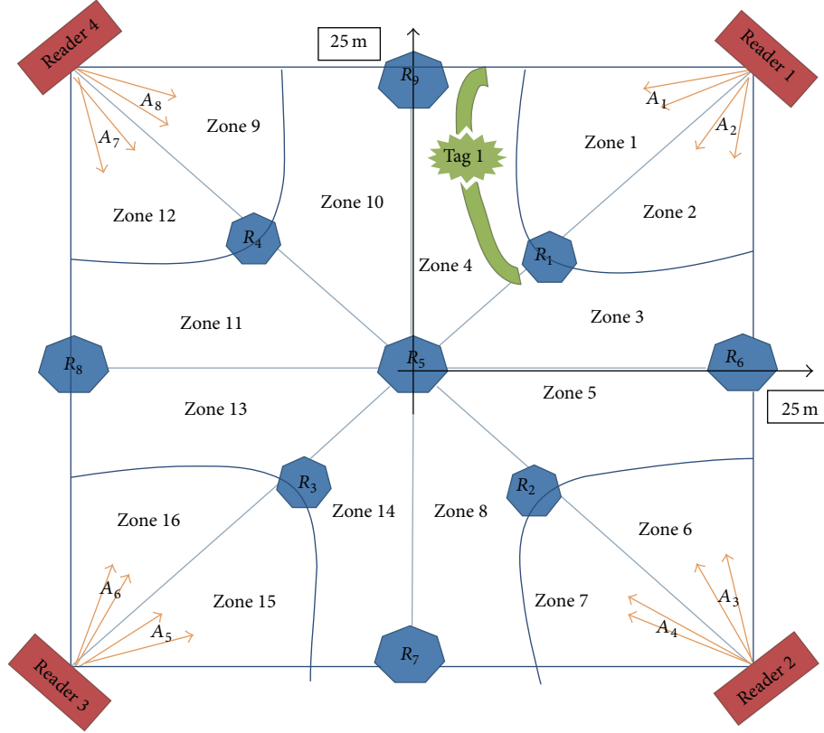
FIGURE 1: Demonstration of RSSI positioning algorithm based on microzones.
