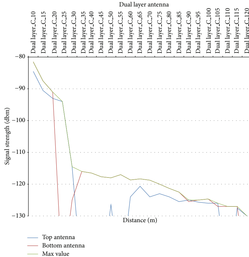
FIGURE 10: Long range detection at test site 3.
