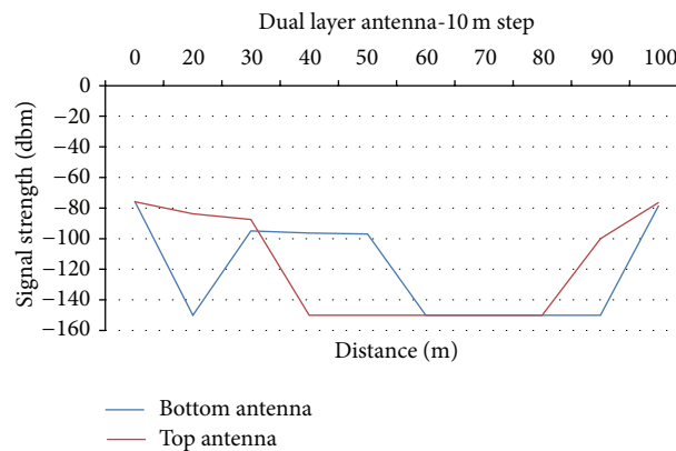
FIGURE 9: Long range detection at venue 2.
