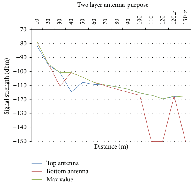
FIGURE 7: Long range detection at test site 1.
