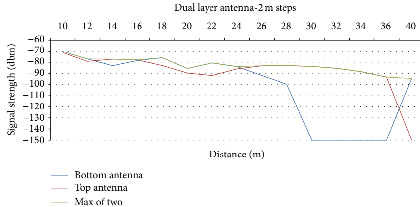
FIGURE 8: Dual layer antenna test -2 m step.
