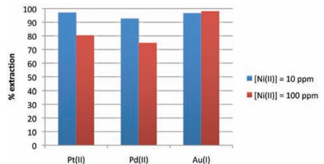
Figure 4—Effects of nickel on the extraction efficiency of PGMs (Pt, Pd, and Au) (contact time: 2 hours; rotational rate: 105 r/min; adsorbent concentration: 15 g/l; temperature: 25°C; pH: 10.75; Cu: 55 ppm; CN: 200 ppm; SCN: 75 ppm; PGMs: 1.33 ppm)
