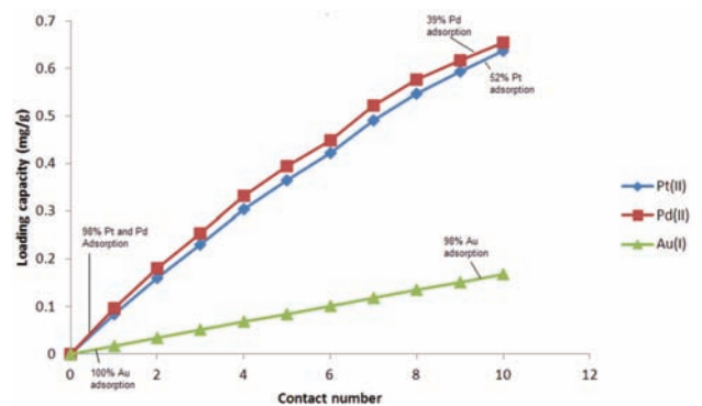
Figure 6—Consecutive loading of Pt, Pd, and Au onto activated carbon from a fresh synthetic BM-PGM solution at 2-hour intervals (adsorbent concentration: 10 g/l; temperature: 25°C; Cu: 10 ppm; Ni: 10 ppm; pH: 9.5; CN: 132 ppm; SCN: 100 ppm; PGMs: 2.03 ppm; rotational rate: 105 r/min)
