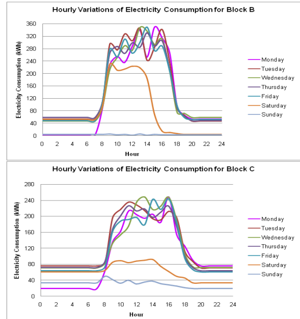
Fig. 6 Week One Electricity Consumption Hourly Variations
