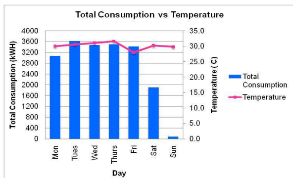
Fig. 10 Relationship between Temperature and Consumption
