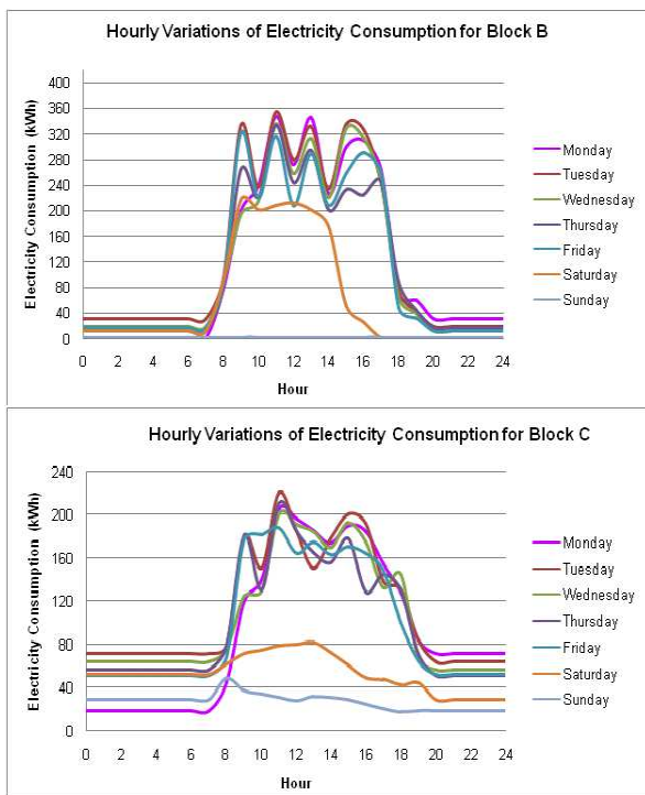
Fig. 5 Semester Break Electricity Consumption Hourly Variations
