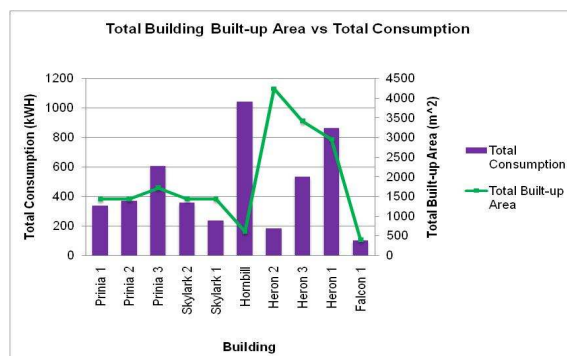
Fig. 9 Relationship between Building Built-Up Area and Total Electricity Consumption
