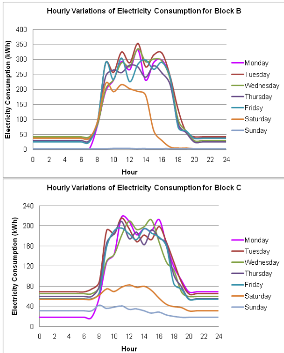
Fig. 4 Tuition Free Week Electricity Consumption Hourly Variations
