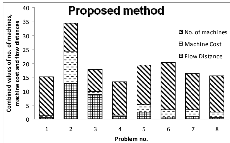
Fig. 7 Problem number versus combined values of number of machines, machine cost, and flow distances for the proposed method
