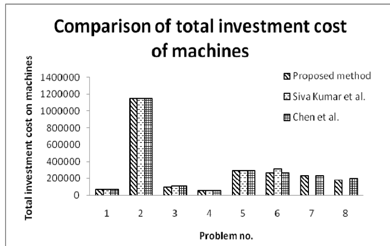
Fig. 4 Comparison of total investment cost of machines
