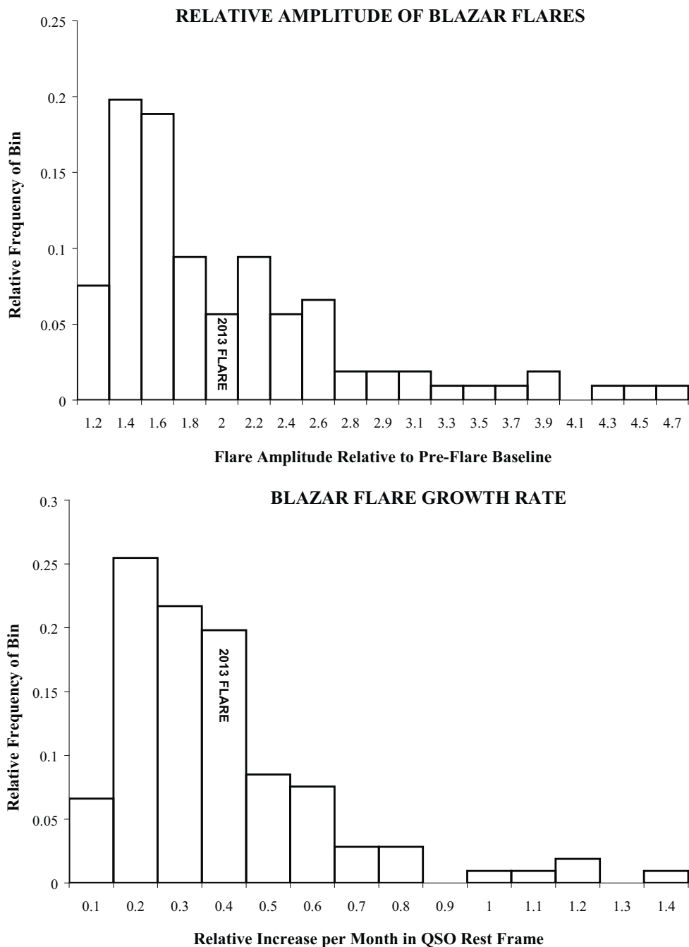
Fig. 3.— Comparison of the 2013 flare in the Mrk 231 to the distribution of flare parameters in the Teräsraanta et al. (2004) blazar sample. The top frame shows the distribution of the normalized flare amplitude, P/Q . The bottom frame is the time rate of increase in normalized units, \dot{S} = (P/Q)/(\text{rise time}) , from the quiescent baseline to the flare peak (units are months -1 ). Two flares from Teräsraanta et al. (2004) are very abrupt and are off the bottom histogram, to the right.
