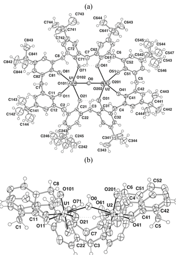
Fig. 1 (a) The anion of 1c , projected normal to the ligand 'plane'. (b) Side-view of the anion, devoid of t -butyl groups. In Table 1, O(a) are the set O(21,31,61,71) and O(b) O(11,41,51,81).
