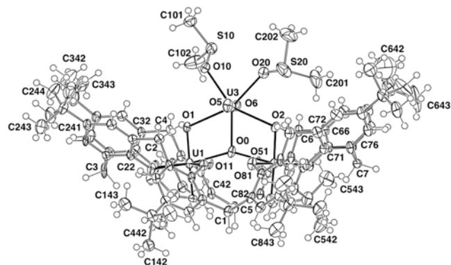
Fig. 5 The anion of 2 , projected normal to the U 3 plane. About U(3) the sets O(a) and O(b) denote O(1,2) and O(10,20)
