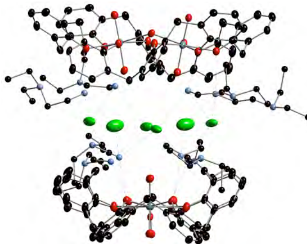
Fig. 2 A simplified view (omitting t -butyl groups and hydrogen atoms, and removing thermal ellipsoids for the Et 2 NCH 2 CH 2 NH 3 + cations) of the hydrogen bonded capsule formed in 1c involving two calixarene complex anions encompassing eight Et 2 NCH 2 CH 2 NH 3 + cations and six chloride anions.
