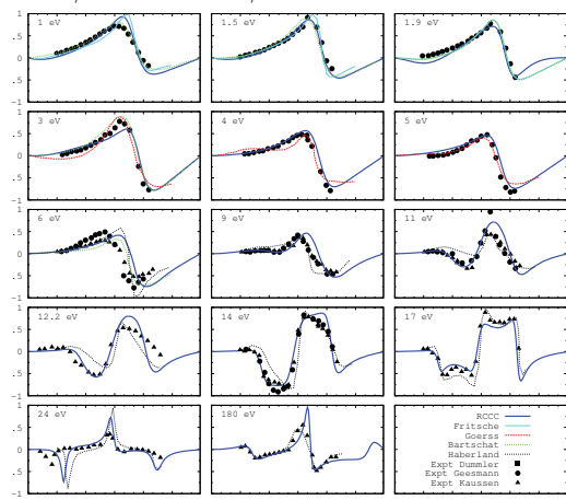
Figure 1. Spin asymmetry function for 6p^2P_{1/2}^o \rightarrow 6p^2P_{1/2}^o elastic electron scattering on thallium. Theory and experiment references are listed in [2].
