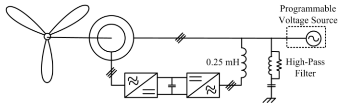
Figure 5. Schematic circuit diagram of the simulated network.
