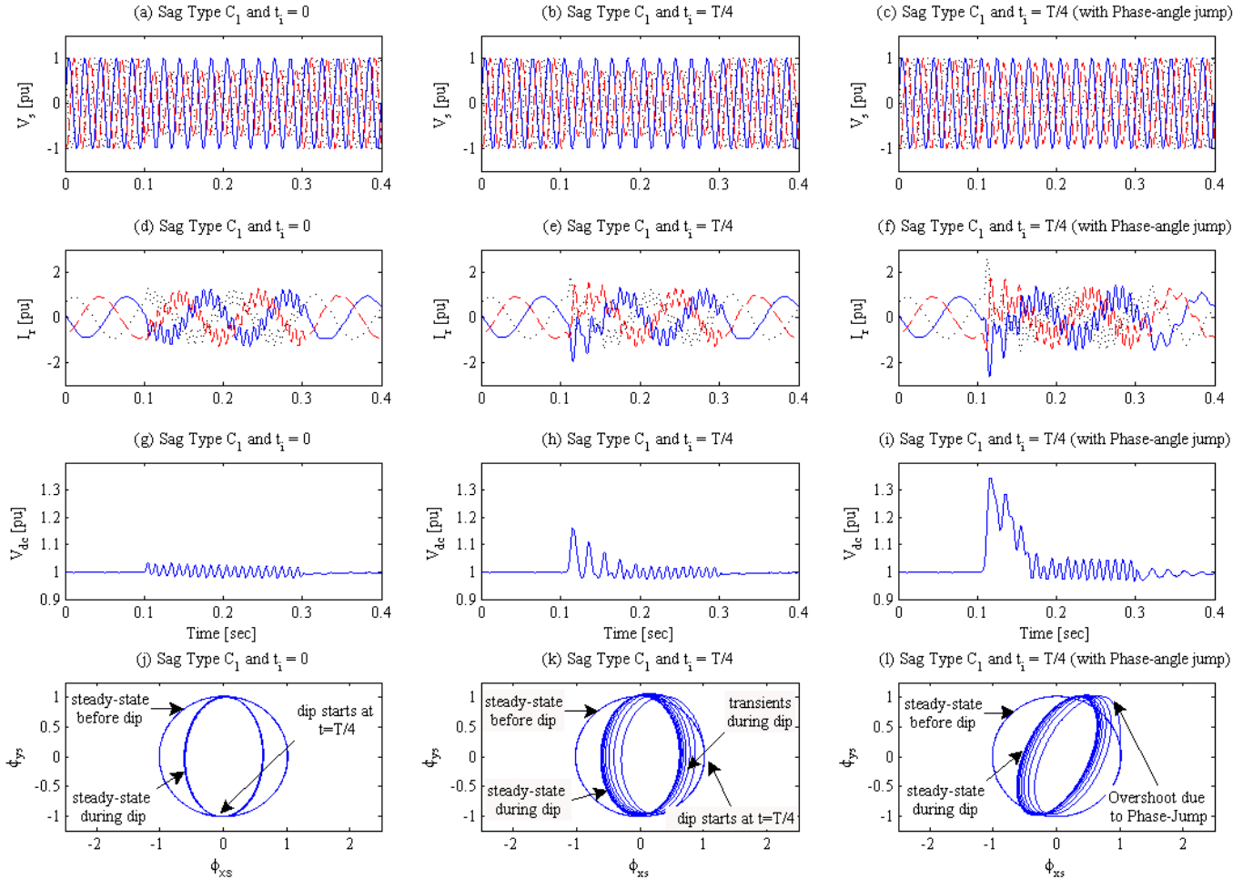
Figure 8. Simulation results for 60% type C voltage sag with different initial point-on-wave instants, without and with phase-angle jump.
