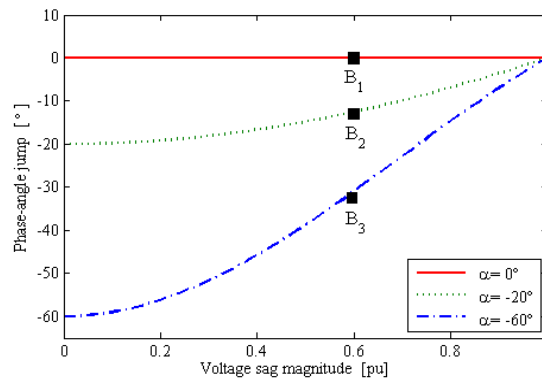
Figure 3. Voltage sag magnitude vs. phase-angle jump for various impedance angles.
