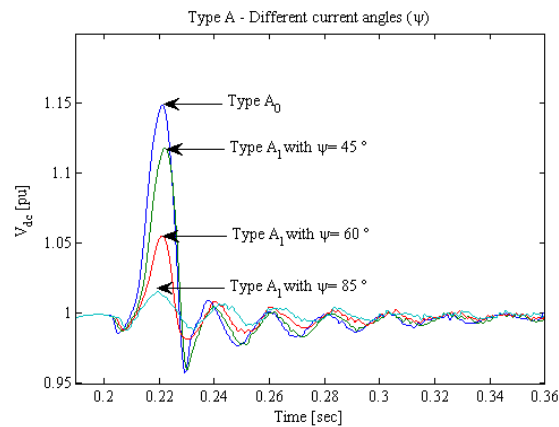
Figure 7. Influence of the fault current angle, \psi , on the dc-link voltage during the voltage recovery process.
