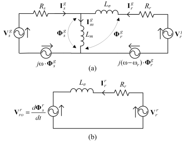
Figure 4. (a) "T-form" equivalent circuit of the machine.
