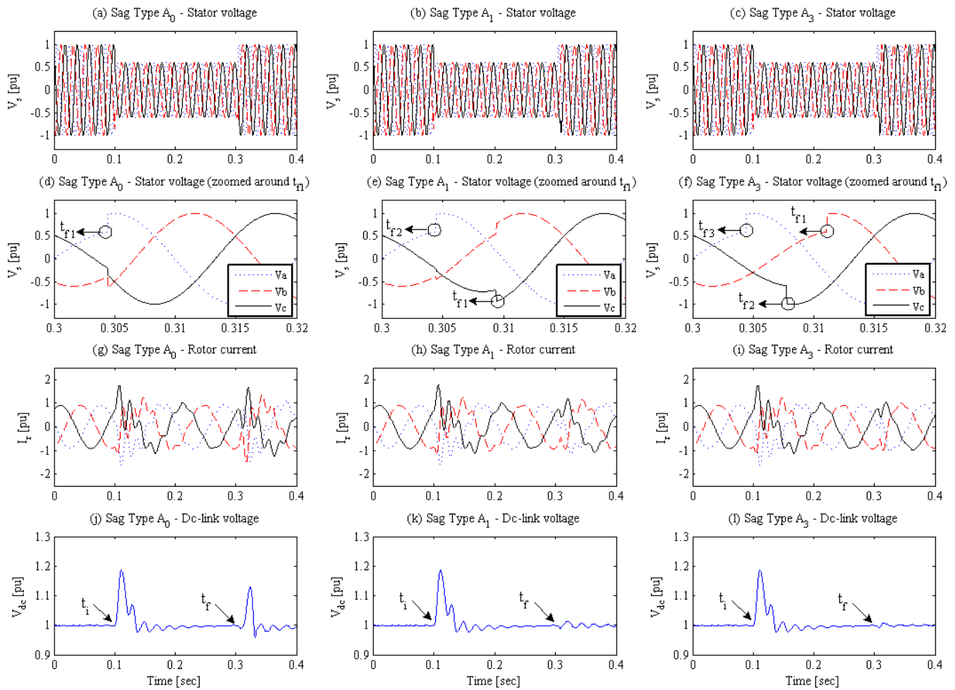
Figure 6. Simulation results for three-phase faults (type A) with different possibilities of the voltage recovery.
