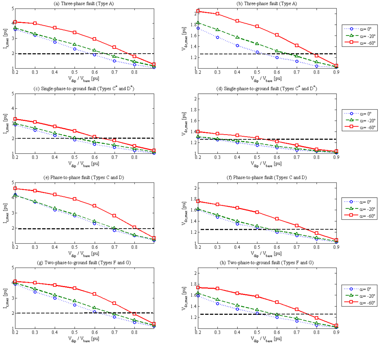
Figure 10. Influence of the sag depth on the transient response of DFIG-based wind turbine subjected to different types of faults (typical safety margins are shown with dashed horizontal lines).
