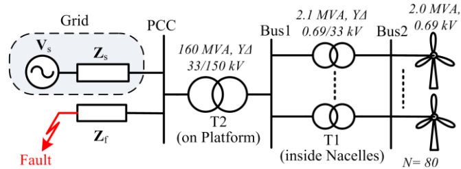
Figure 2. Voltage divider model ( italic figures are the real parameters for Horns-Rev Wind Farm and ‘N’ is the total number of wind turbines. )
