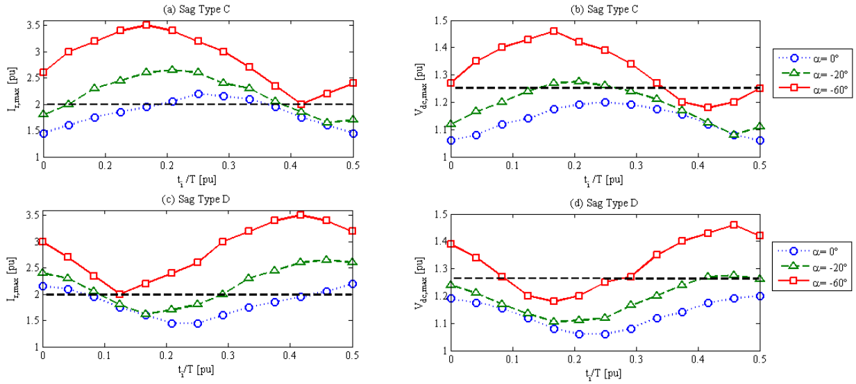
Figure 9. Influence of the initial point-on-wave instant on the transient response of DFIG-based wind turbines subjected to phase-to-phase faults, i.e., sag types C and D (typical safety margins are shown with dashed horizontal lines).
