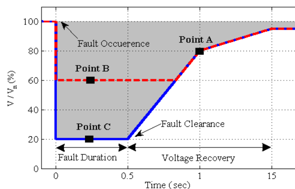
Figure 1. Fault ride-through requirements of wind farms at the PCC - Spanish Grid Code.
