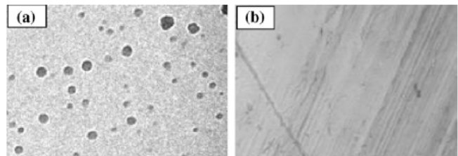
Fig. 10 SEM picture of 5 wt.% clay filled composite (a)before (b) and after degassing [8]
