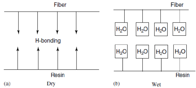
Fig. 3: a) H-bonding between fibre and resin in dry condition b) water acts as separating layer that leads to separation between fibre and resin in wet condition [6]
