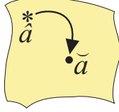
Fig. 1 An ambiguity pull-in region of z = \tilde{a} .
