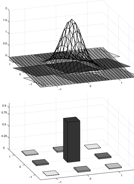
Fig. 6 (top) The two-dimensional pdf of the 'float' solution \hat{a} situated over the bootstrapped pull-in regions; (bottom) the two-dimensional pmf of the integer bootstrapped solution \check{a}_B .
