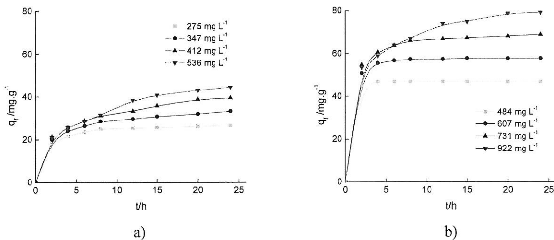
Fig. 3. Effect of stirring time on the adsorption of a) Zn^{2+} and b) Cd^{2+} using ZM1 (weight of adsorbent = 1 g, T = 25\text{ }^{\circ}C ; pH_{in} = 5 ).
