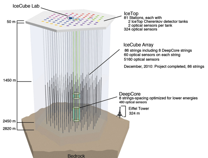
FIG. 1 (color online). Three-dimensional view of the IceCube detector layout. This work was based on the 40-string configuration which was half of the completed detector. The 40-string configuration was operational from April 2008 to May 2009.
