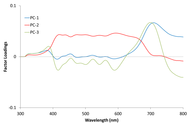
Fig.5. Loading plot for window tint model
